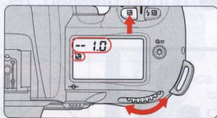
Electronic analog exposure display
